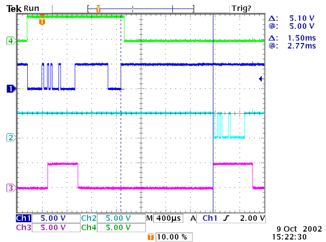
Figure 2-11. Binary Command Write then Read
